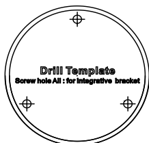
Figure 2-11 Drill Template
